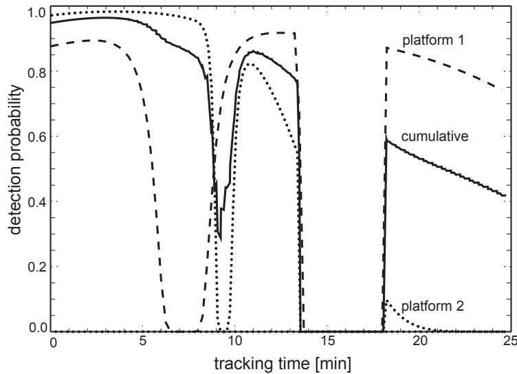
Fig. 2.7. GMTI tracking: detection probability of the individual sensors and the mean accumulated detection probability as a function of the tracking time.
